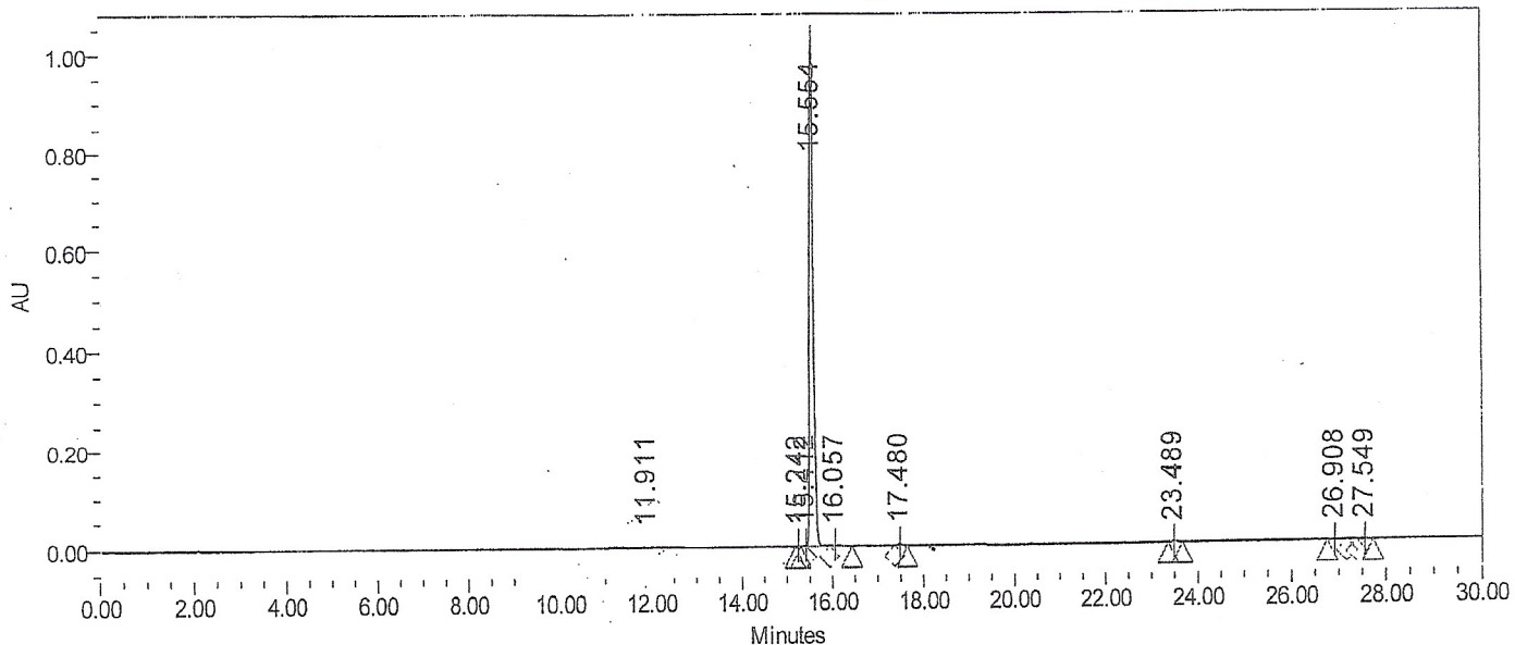
Auto-Scaled Chromatogram
